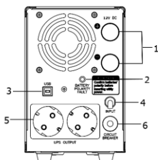
12VDC(500/800VA)
